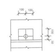
PLAN 1-1 SCALE 1:50
