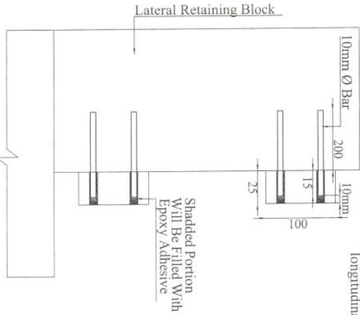
EXPANSION JOINT ANCHOR DETAIL NOT TO SCALE
