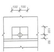
PLAN 1-1 SCALE 1:20
