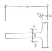
SECTION 5-5 SCALE 1:50
