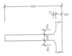
SECTION 5-5 SCALE 1:50
