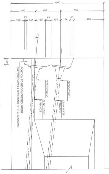
DETAIL OF END BLOCK (SHOWING POSITION OF CABLE ANCHORAGES) SCALE 1=20
