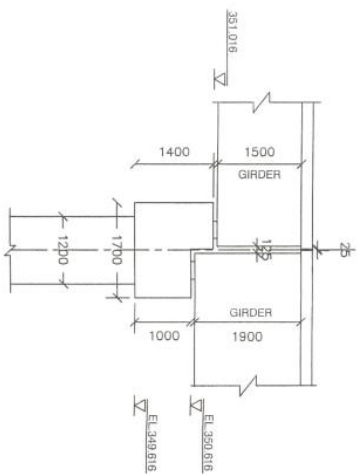
PIER 01 & PIER 04 TRANSOM ELEVATION VIEW
