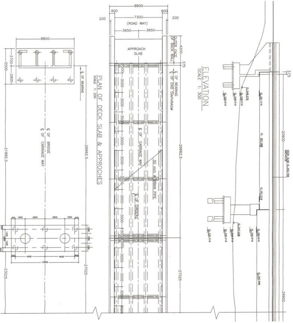
PLAN SHOWING SUB-STRUCTURE SCALE 1: 200
