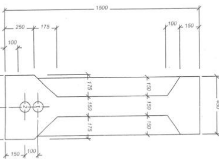
SECTION 3-3 SCALE 1=20
