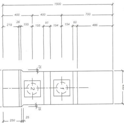
ELEVATION 2-2 SCALE 1=20
